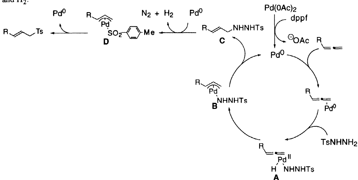
Scheme 1. Hydrosulfination Reaction Mechanism
